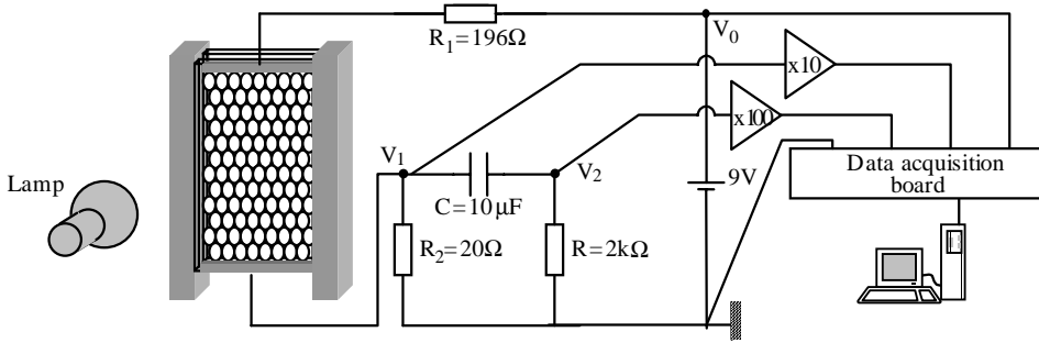
Fig. 1 – Experimental set-up.
