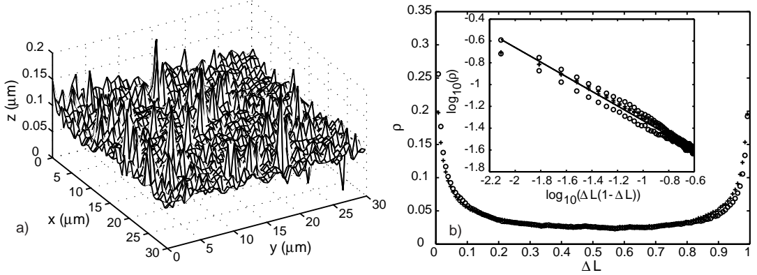
Fig. 4 – (a) AFM picture of the bead surface and (b) density \rho as a function of the relative difference \Delta L with L_2 = 128 . \circ correspond to row averaging and + correspond to column averaging. Inset: \log_{10}(\rho) as a function of \log_{10}(\Delta L(1 - \Delta L)) . The straight line corresponds to a fit using eq. (4).
