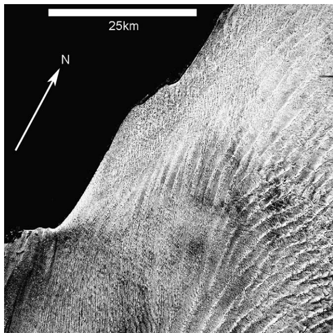
Fig. 3. A 45 \times 50 km section of the Namib desert at 15^{\circ}\text{E} , 25^{\circ}\text{S} , observed by the Shuttle Imaging Radar (SIR-C) mission in 1994 (scene PR44419) – brightness is inverted for clarity. The bright dark South Atlantic Ocean is at left, with a strip of small coastal dunes (spacing 500–600 m) grading into much larger linear dunes inland (spaced by 1.5–2.5 km), suggesting echoing the expected trend of the atmospheric boundary layer thickness may exhibit a similar trend.
