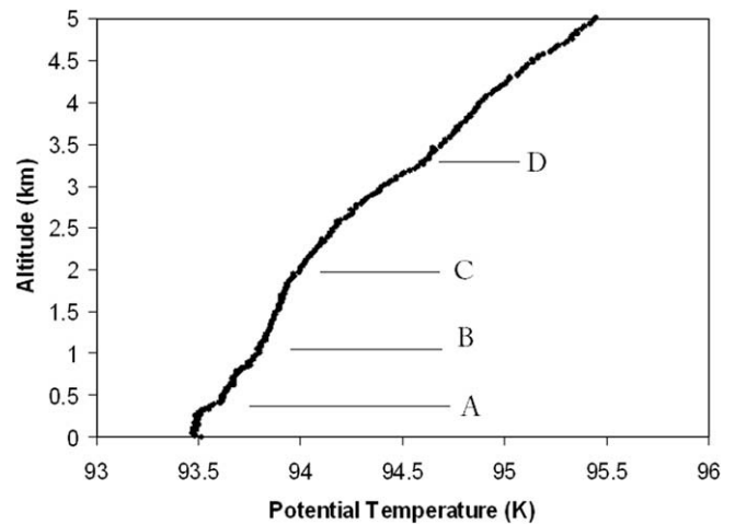
Fig. 2. The near-surface potential temperature profile derived from Huygens data (Tokano et al., 2006). The constant \Theta region 0–300 m identified in that paper as the boundary layer is clearly seen (A); two additional steps in the profile at ~0.9 km and ~2 km (B and C) were suggested by Griffith et al. (2008) as suggesting a rather thicker, older boundary layer (C) had been modified subsequently (A and B). An additional inflection is seen at ~3.3 km (D).
