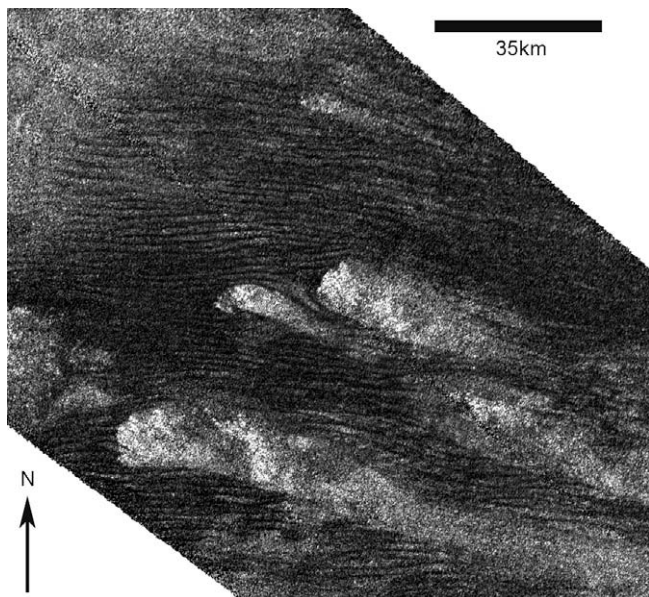
Fig. 1. A section of the T 41 Titan SAR swath at 180°W, 25°S, southeast of the Huygens landing site, showing typical dune spacing. Although dark topographic obstacles can interrupt the dunefield, the characteristic ~3 km spacing is evident.
