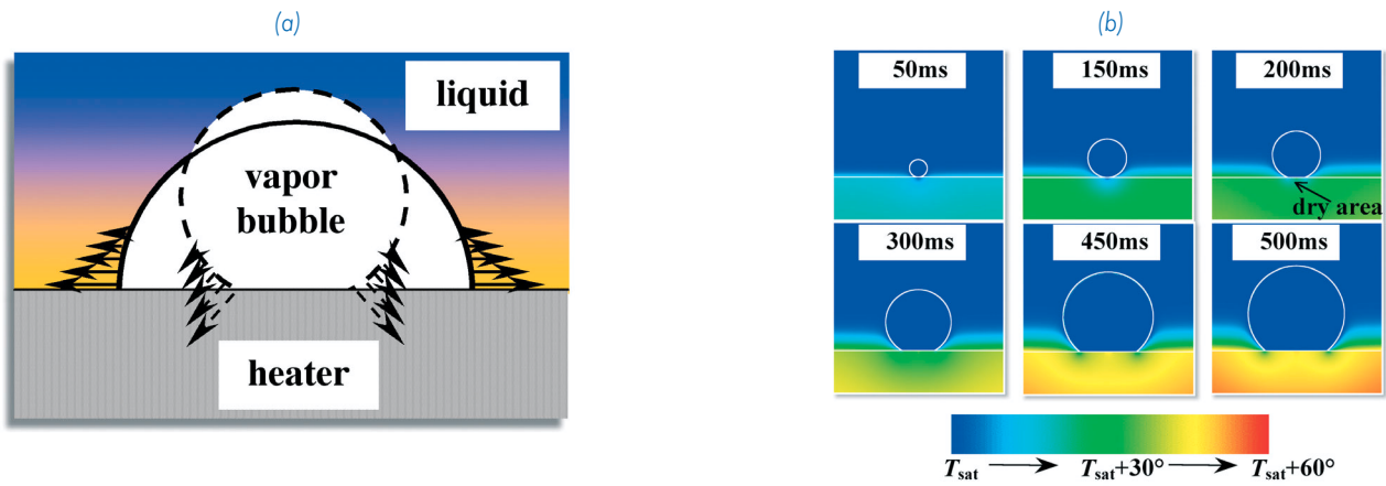
Figure 1. Vapor bubble spreading under the influence of vapor recoil.
