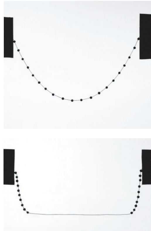
Fig. 2: Shape of a soft solid thread with either a homogeneous distribution of mass (provided by a regular spacing of 10 mm between the millimetric plumbs fixed on it), or an non-homogeneous one; in the second photo, the same number of plumbs is localised close to the fiber ends (distance between plumbs of 5 mm). The distance between the attachment points and the total length of the thread are 13 cm and 20 cm, respectively.
