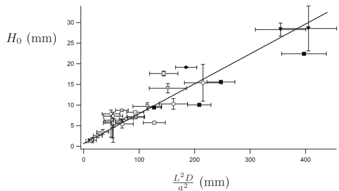
Fig. 6: Final depth H_0 of U-filaments, as a function of their geometry. Filaments are made of silicone oil of viscosity \eta = 1 Pa s (circles), 10 Pa s (squares) and 100 Pa s (diamonds), or honey of viscosity \eta = 5 Pa s (triangles). Their initial length is L \approx 12 mm (white symbols), L \approx 25 mm (grey symbols) and L \approx 57 mm (black symbols). The depth is observed to scale fairly well with the geometrical quantity DL^2/a^2 , as expected from eq. (4).
